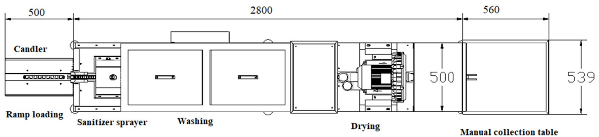
ZYX-J1-1 egg washer product code:200AS capacity: 2000 eggs/hour
